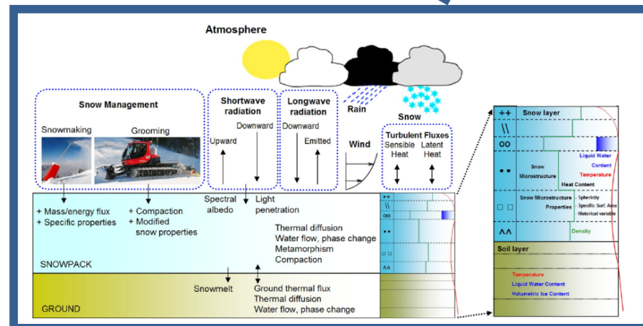
Snowpack modelling
